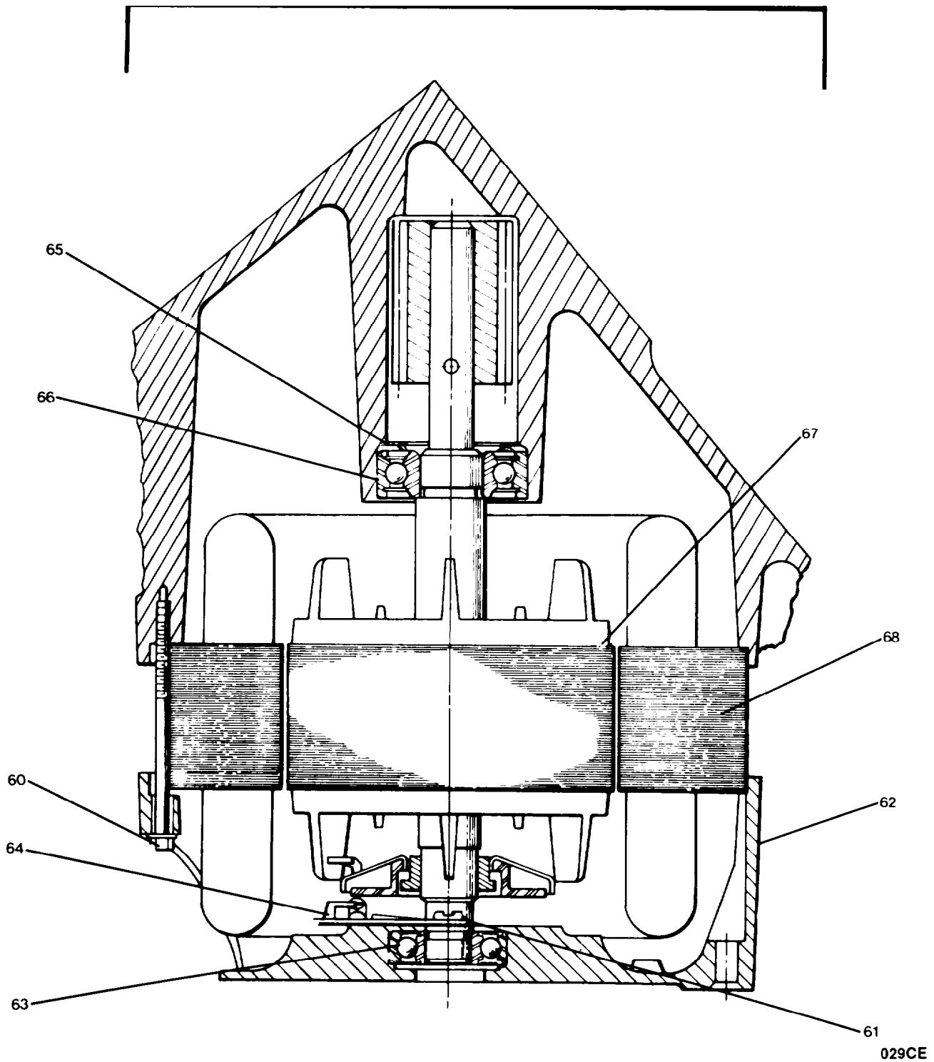
Detail E Motor Parts
