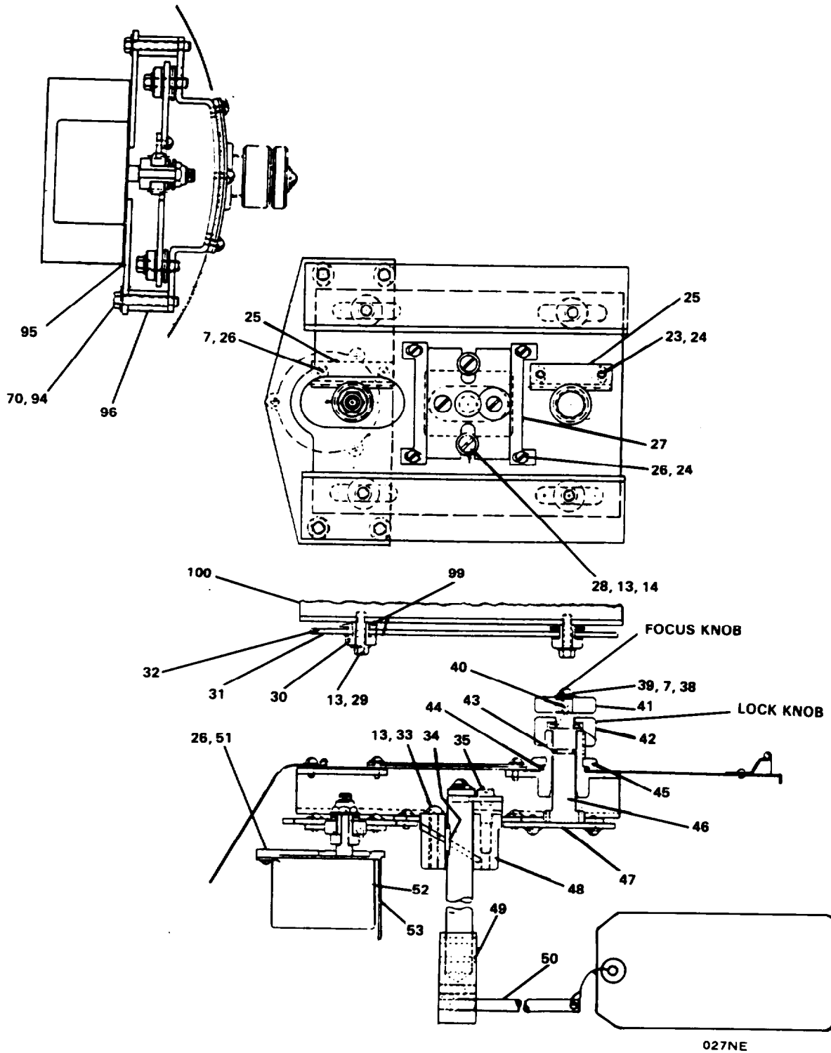
FIGURE 383. Drum Assembly (Sheet 4 of 4).
