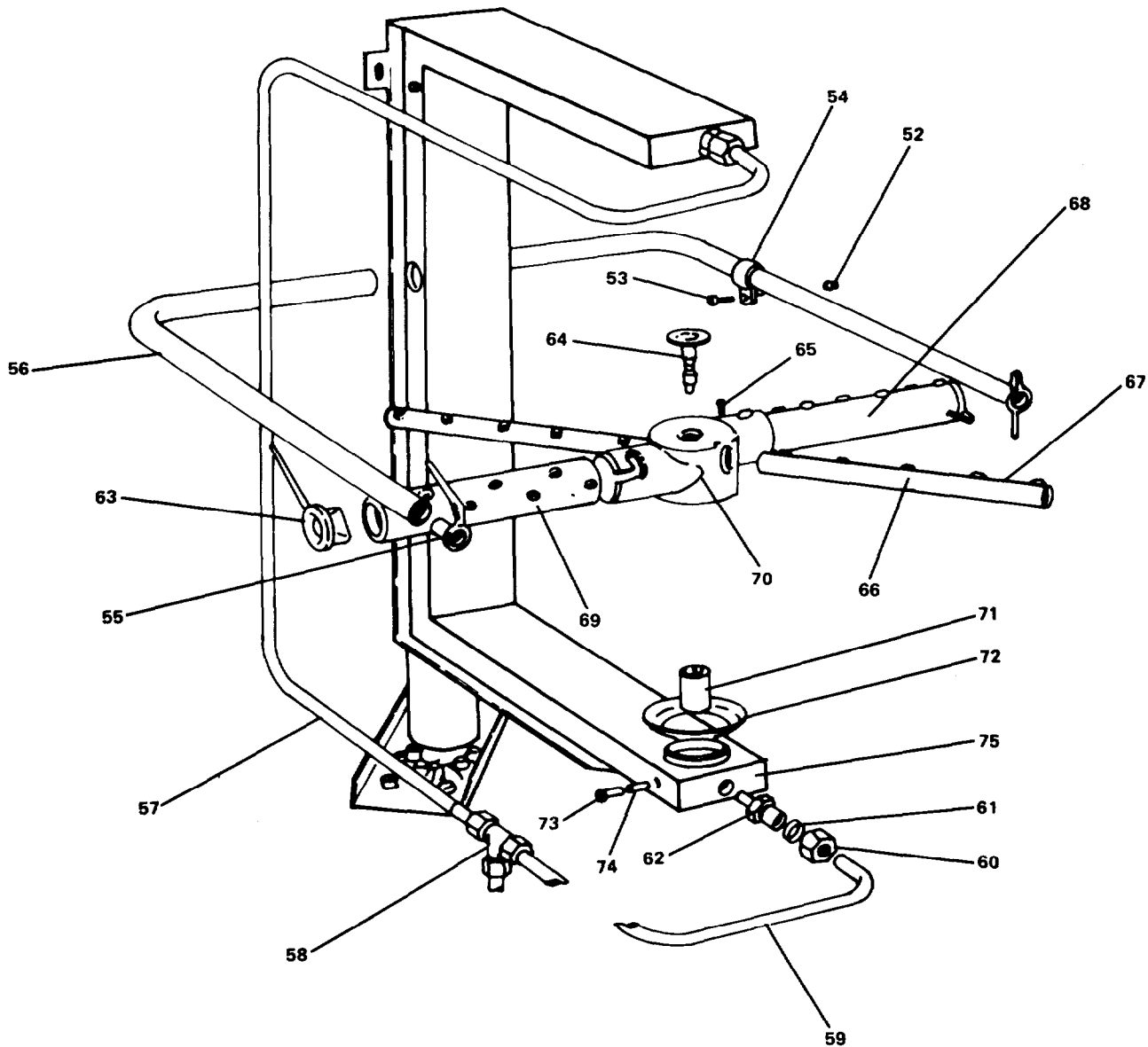
PUMP AND MOTOR ASSEMBLY
