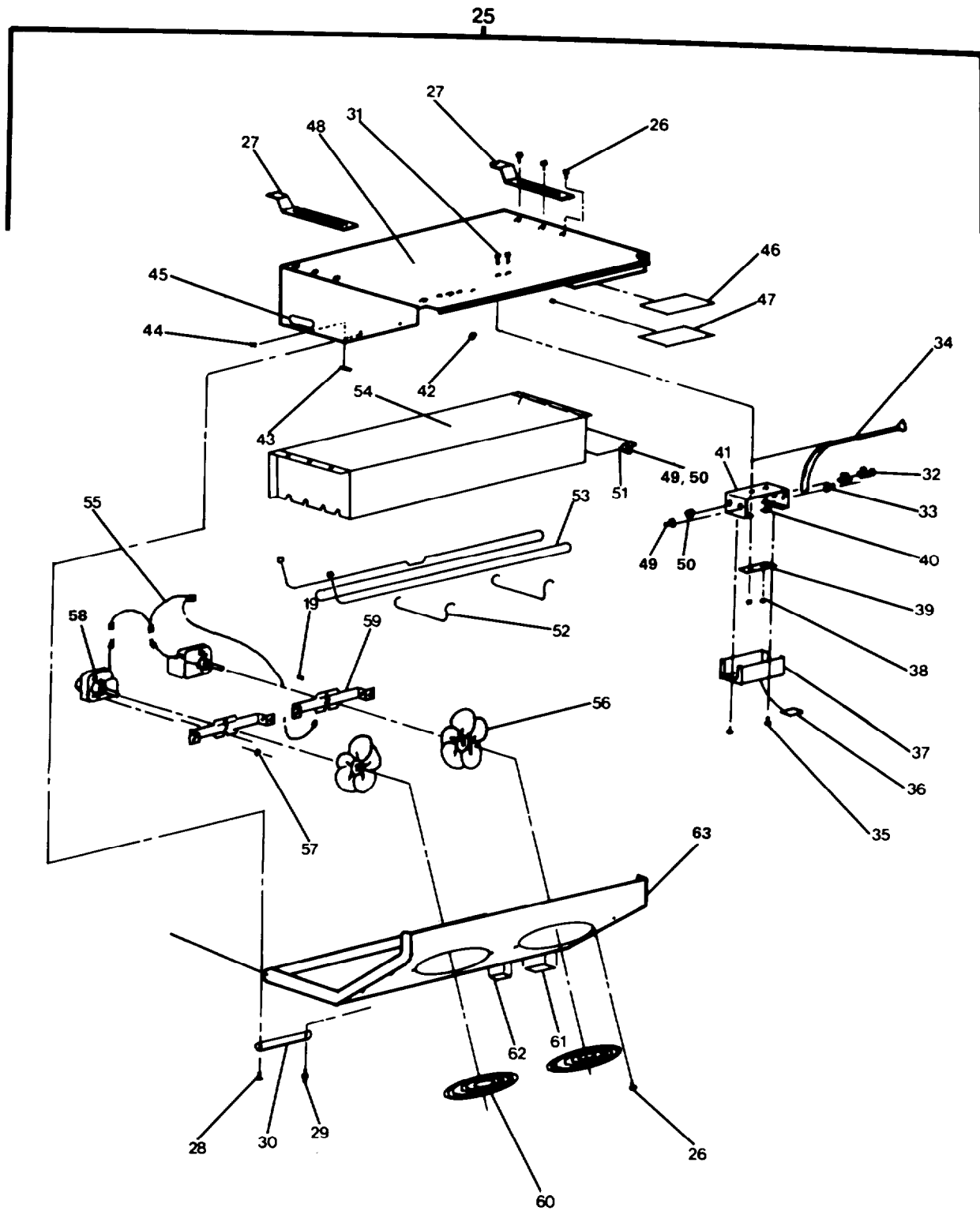
DETAIL A EVAPORATOR COIL ASSEMBLY
