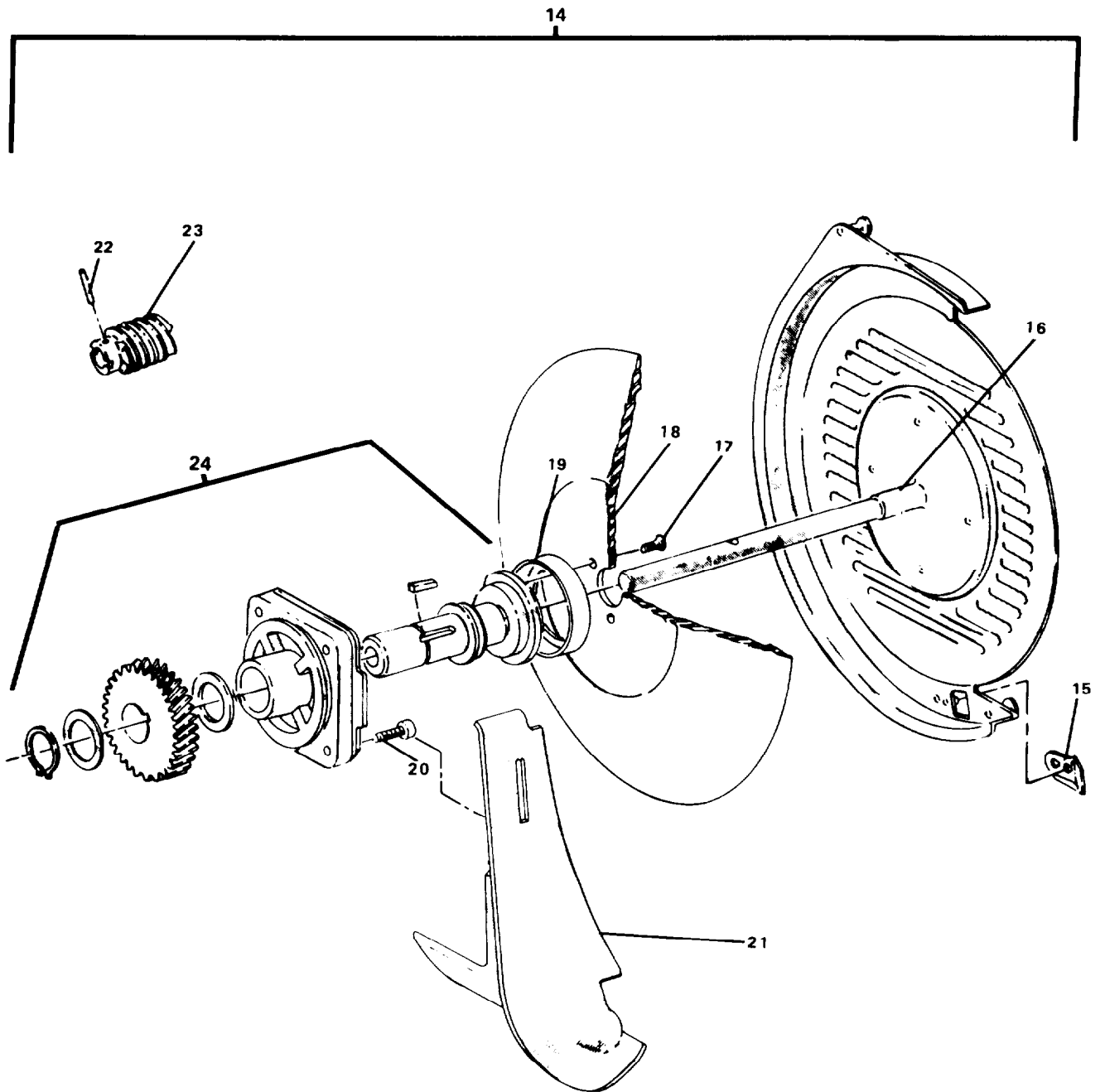
DETAIL B KNIFE UNIT ASSEMBLY
