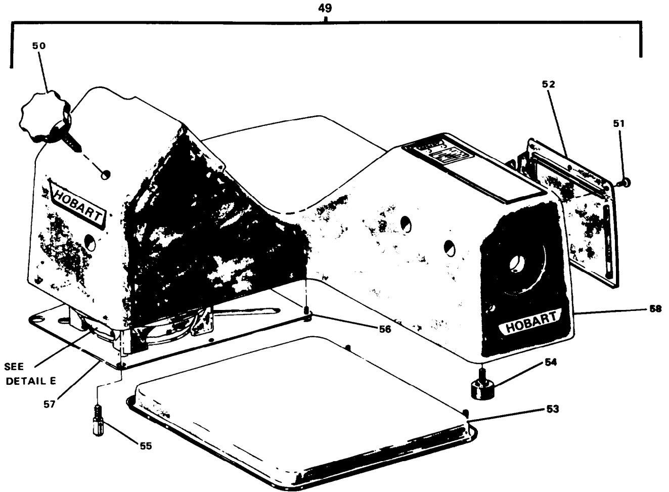
DETAIL D BASE UNIT ASSEMBLY
