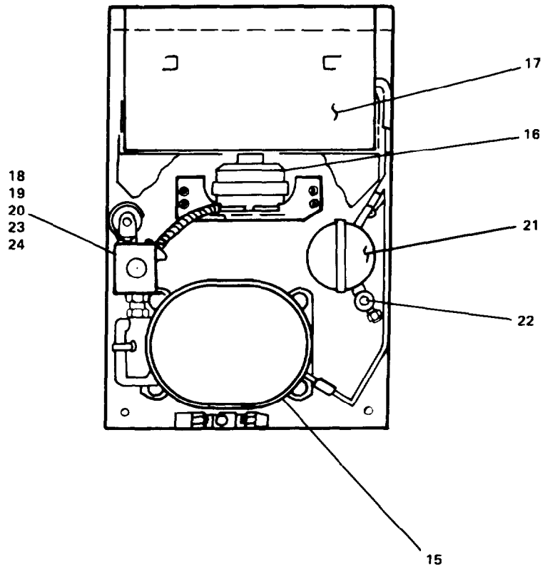
DETAIL A CONDENSER, REFRIGERATION
