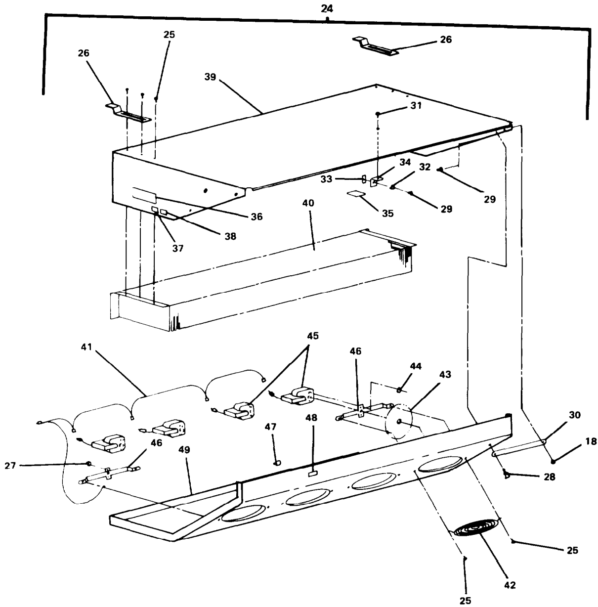
DETAIL A EVAPORATOR COIL, REFRIGERATION
