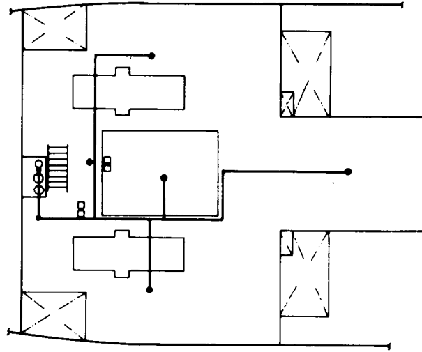
PLAN VIEW MAIN MACHINERY ROOM BELOW MAIN DECK
