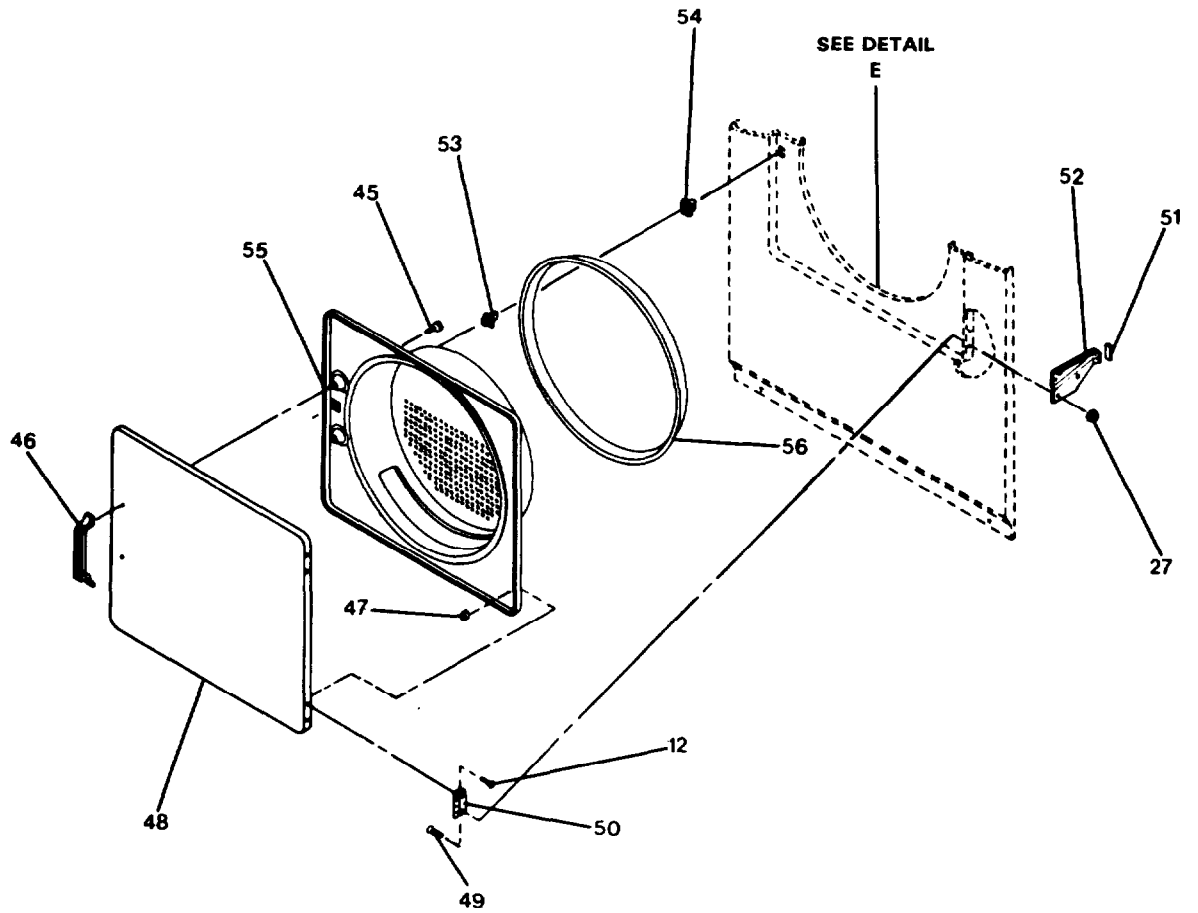
DETAIL D LOADING DOOR ASSEMBLY
