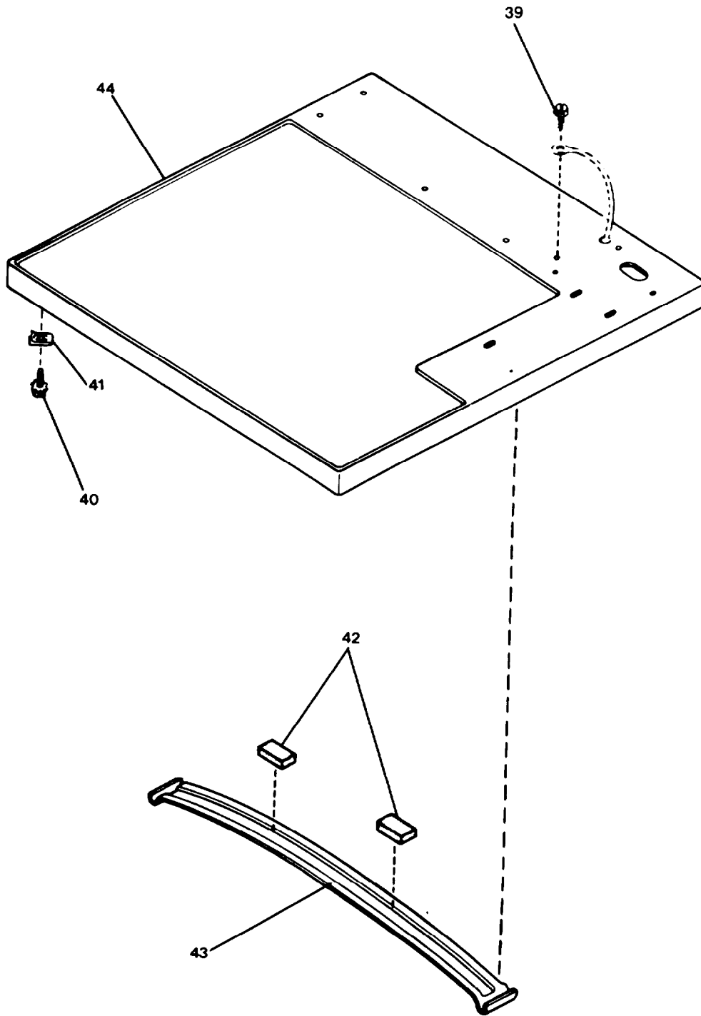
DETAIL C CABINET TOP ASSEMBLY
