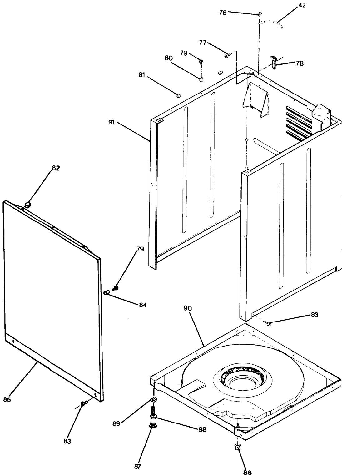
DETAIL E FRONT PANEL, CABINET, AND BASE
