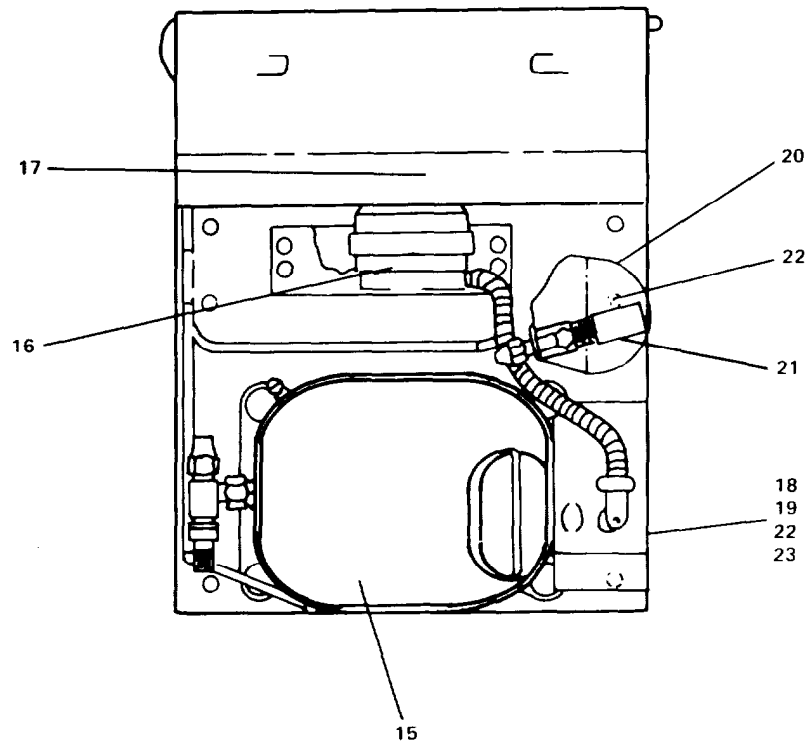
CONDENSER, REFRIGERATION
