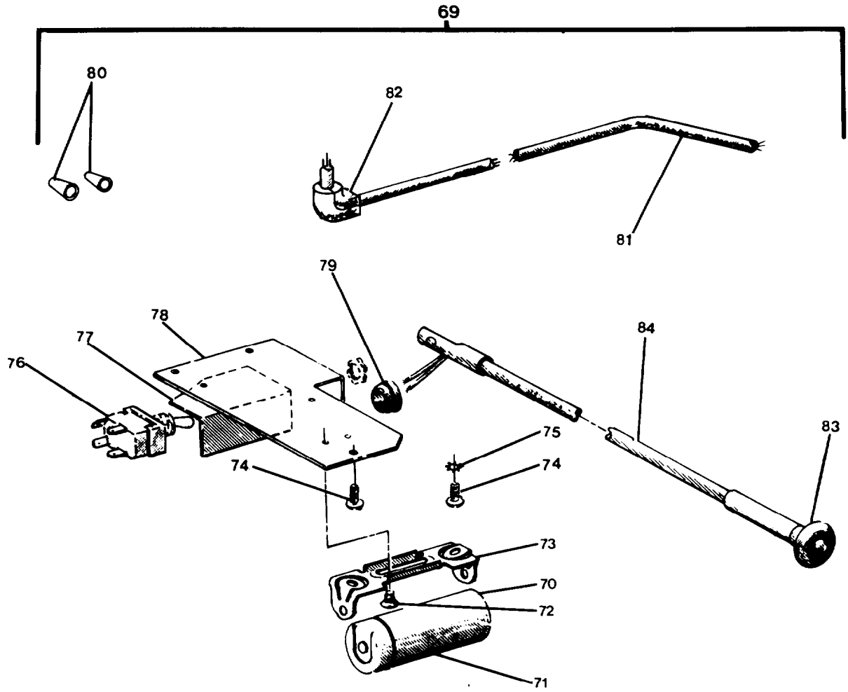
DETAIL F ELECTRICAL UNIT ASSEMBLY
