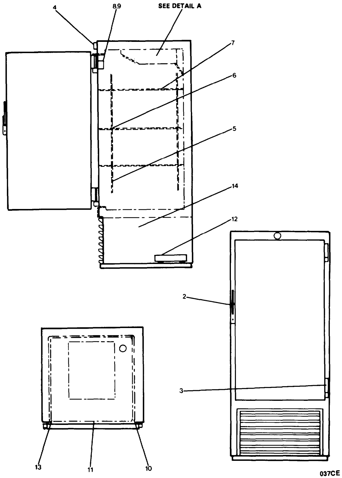
FIGURE 413. Freezer, Mechanical, Food (Sheet 2 of 4).
