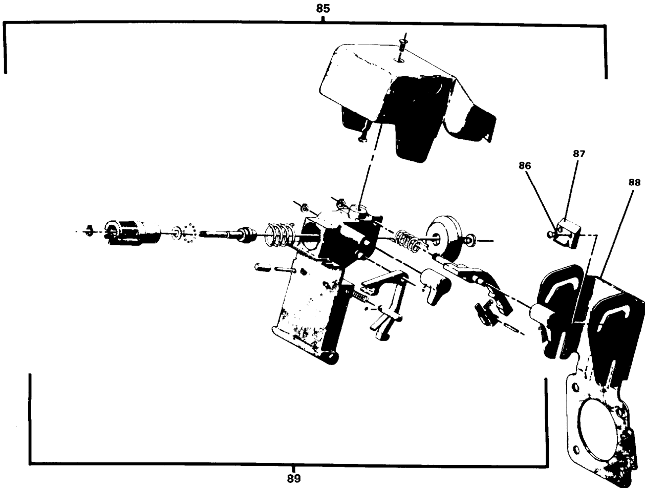
DETAIL G KNIFE SHARPENER UNIT ASSEMBLY
